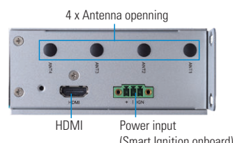
▲ Top view (non-PoE SKU)
